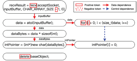
(c) Subgraph of program dependency graph
